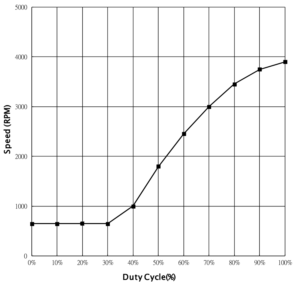
Duty Cycle v.s. Speed curve
