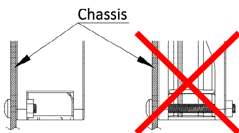
● FLANGE TYPE
