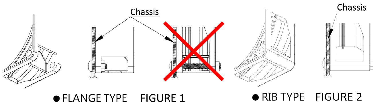
● FLANGE TYPE
