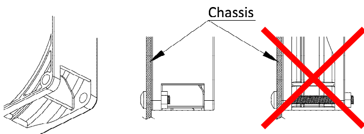
● FLANGE TYPE FIGURE 1
